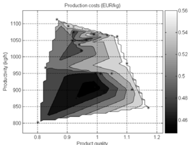
Figure 7. Production Costs in relation to Productivity and Product Quality pPIs for unified production.
